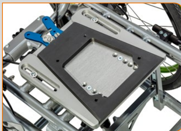
HC-Trapezadapter aus Aluminium HC-trapezium adapter aluminium
