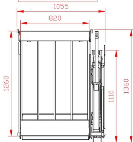
OWU006 IN WORK POSITION RIGHT SIDE
