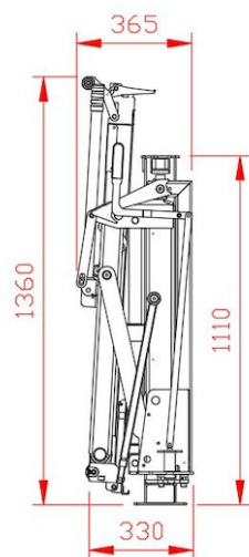
OWU006 IN TRAVEL POSITION RIGHT SIDE
